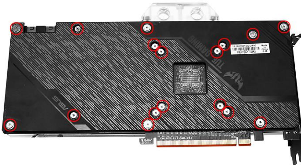
6. Mount the red position screws in the picture
